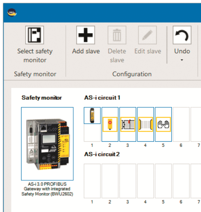
Fig. 2: Simple hardware configuration with ASIMON360
